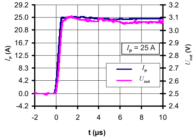
Figure 16: Step response
