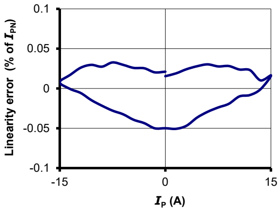
Figure 7: Linearity error
