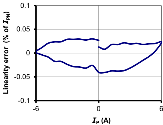
Figure 1: Linearity error
