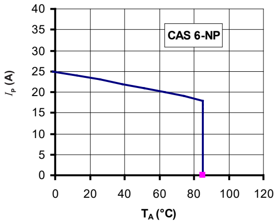
Figure 25: I_P vs T_A for CAS 6-NP
