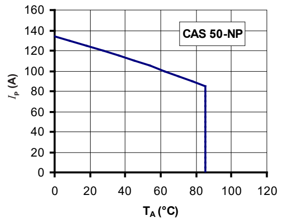
Figure 28: I_P vs T_A for CAS 50-NP
