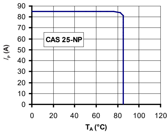
Figure 27: I_P vs T_A for CAS 25-NP
