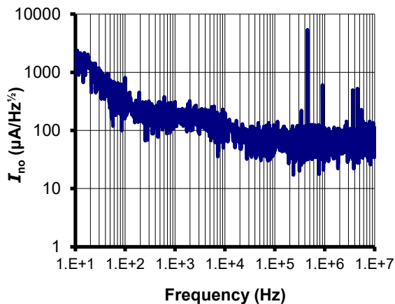
Figure 17: Input referred noise
