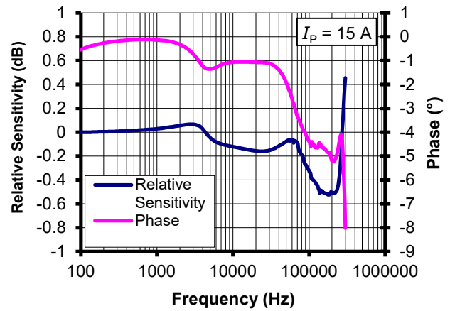
Figure 8: Frequency response
