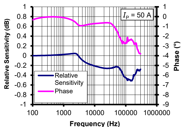
Figure 20: Frequency response
