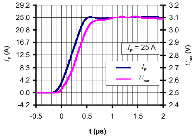
Figure 15: Step response
