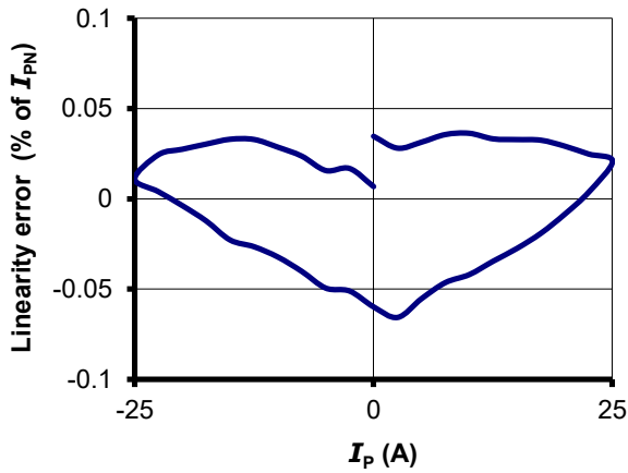
Figure 13: Linearity error
