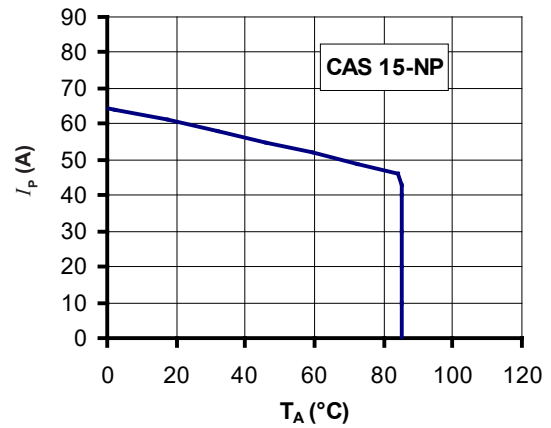
Figure 26: I_P vs T_A for CAS 15-NP
