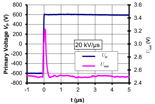
Figure 12: dv/dt
