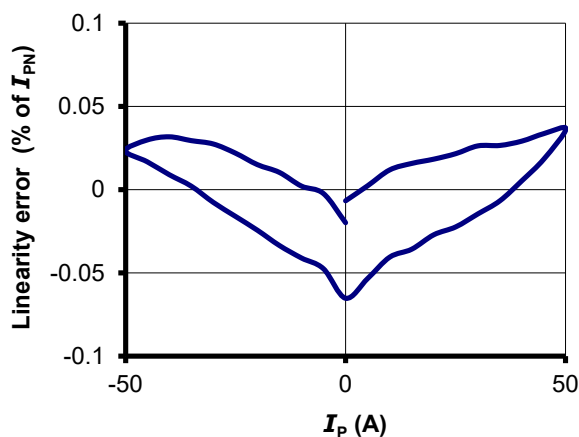
Figure 19: Linearity error
