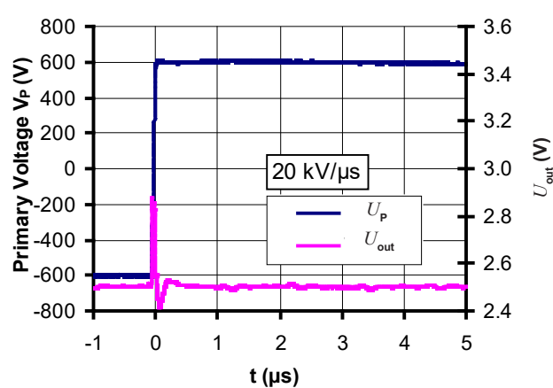
Figure 24: dv/dt
