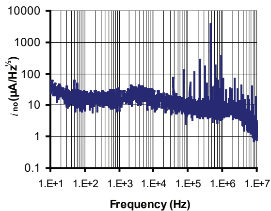
Figure 5 Noise current spectral density referred to primary
