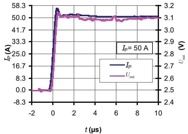
Figure 4: Step response
