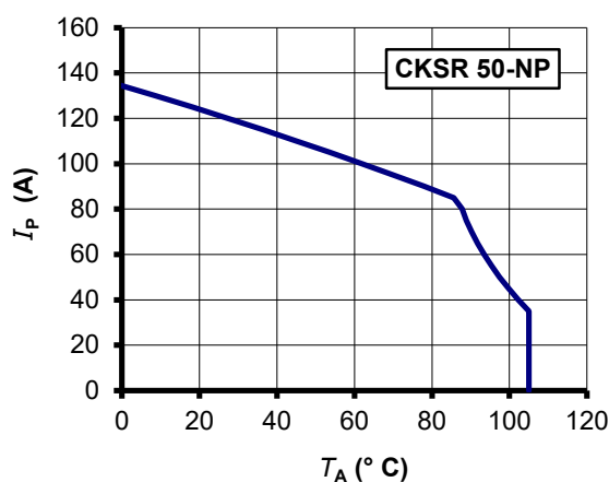
Figure 7: I_p vs T_A for CKSR 50-NP/SP1
