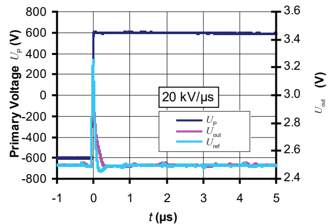
Figure 6: du/dt
