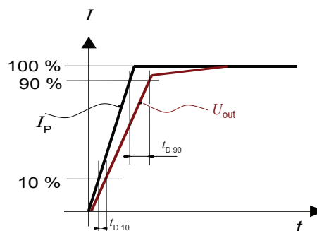
Figure 11: t_{D90} ( delay time @ 90 %) and t_{D10} ( delay time @ 10 %)
