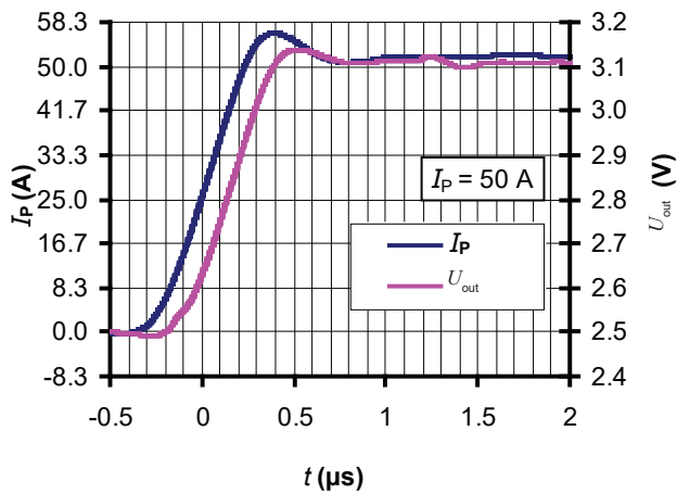
Figure 3: Step response
