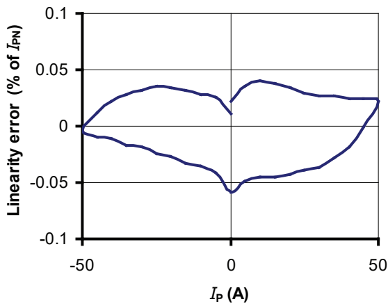
Figure 1: Linearity error
