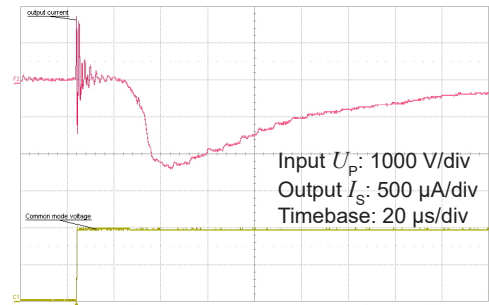
Figure 12: Detail of typical common mode perturbation (2000 V step with 6 kV/μs, R_M = 100 \Omega )
