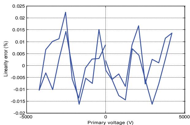
Figure 17: Typical linearity error
