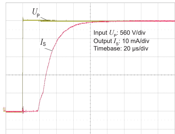
Figure 6: Typical step response (0 to 2800 V)
