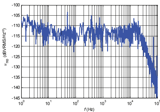
Figure 15: Typical noise voltage spectral density u_{no} referred to primary with R_M = 50 \Omega
