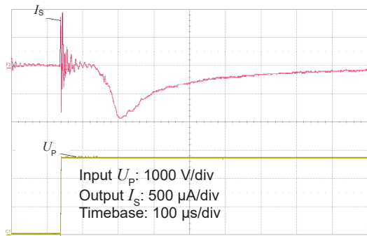
Figure 13: Typical common mode perturbation (2800 V step with 6 \text{ kV}/\mu\text{s} R_M = 100 \Omega )
