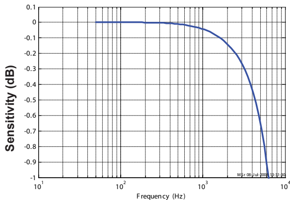
Figure 11, 12: Typical frequency response (detail)
