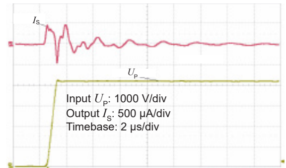
Figure 14: Detail of typical common mode perturbation (2800 V step with 6 \text{ kV}/\mu\text{s} , R_M = 100 \Omega )
