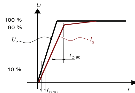
Figure 19: delay time t_{D10} @ 10 % and delay time t_{D90} @ 90 %
