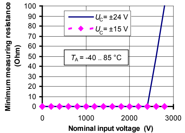
Figure 2: Minimum measuring resistance. For T_A under 80 °C, the minimum measuring resistance is 0 \Omega whatever U_C
