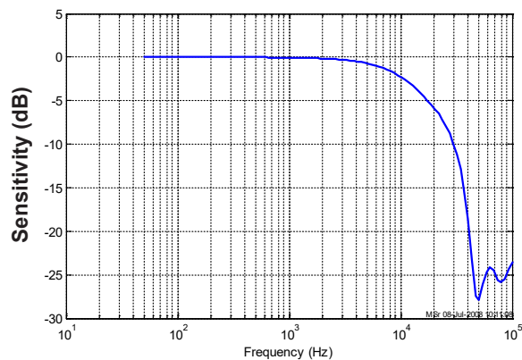
Figure 9, 10: Typical frequency response
