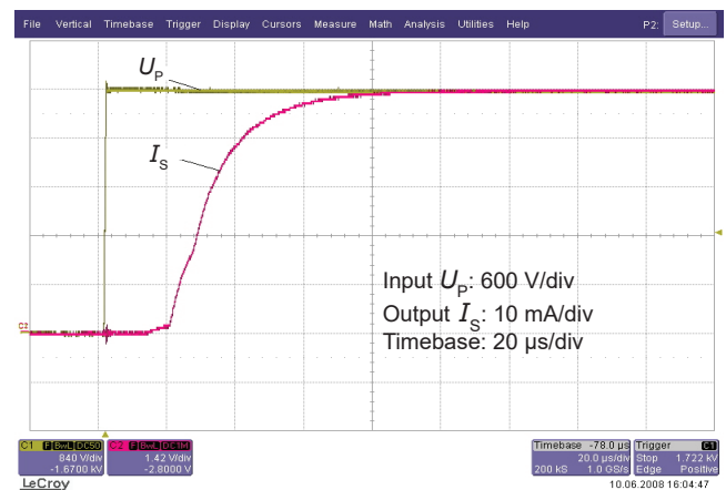
Figure 6: Typical step response (0 to 3000 V)
