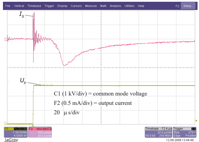
Figure 14: Detail of typical common mode perturbation (2800 V step with 6 kV/μs, R_M = 100 \Omega )
