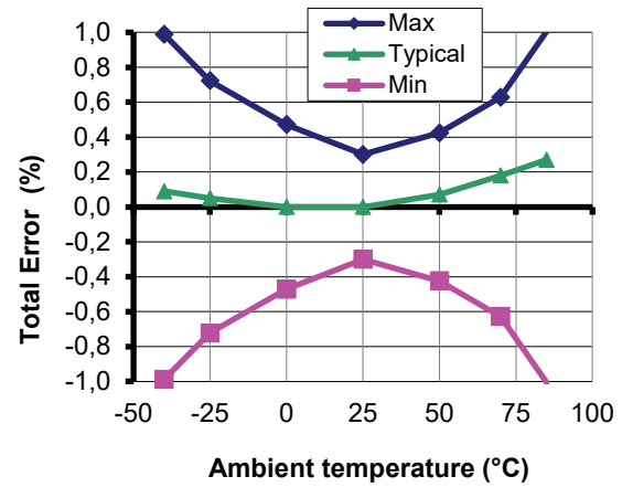
Figure 4: Total error in temperature
