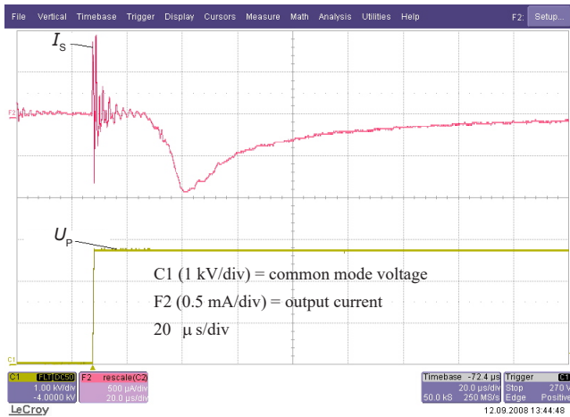
Figure 13: Typical common mode perturbation (2800 V step with 6 kV/μs, R_M = 100 \Omega )
