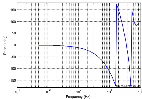
Figures 9, 10: Typical frequency response
