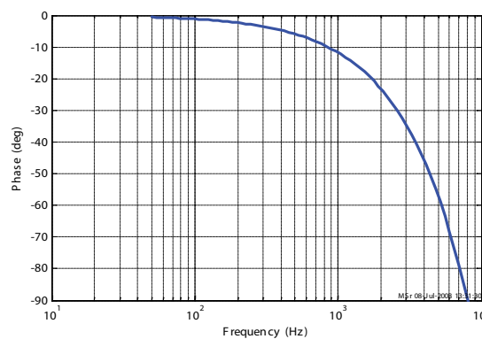
Figures 11, 12: Typical frequency response (detail)
