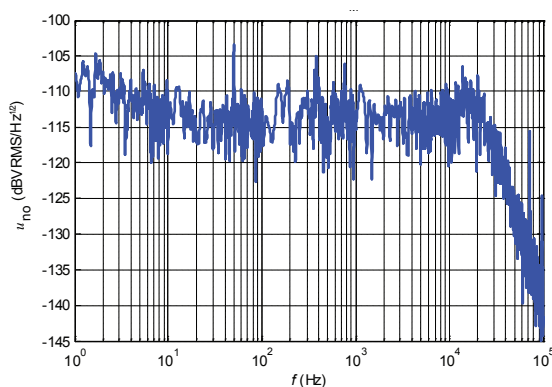
Figure 15: Typical noise voltage spectral density referred to primary with R_M = 50 \Omega
