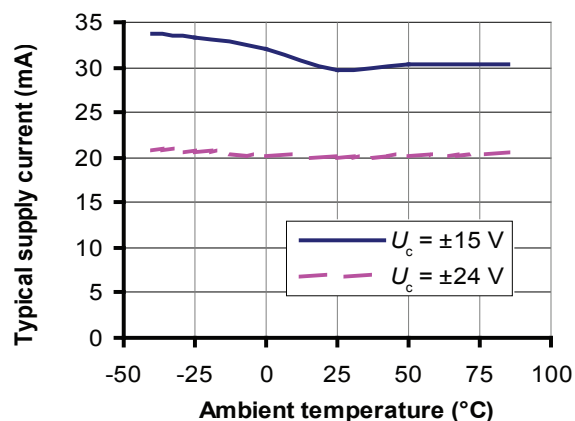
Figure 8: Supply current function of temperature
