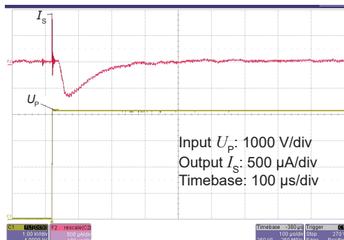
Figure 11: Typical common mode perturbation (4200 V step with 6 \text{ kV}/\mu\text{s} R_M = 100 \Omega )
