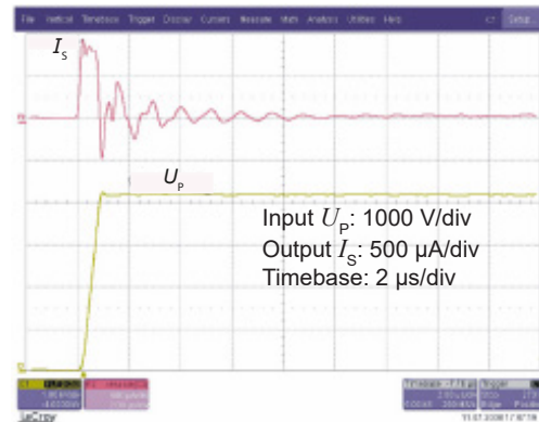
Figure 12: Detail of typical common mode perturbation (4200 V step with 6 \text{ kV}/\mu\text{s} , R_M = 100 \Omega )
