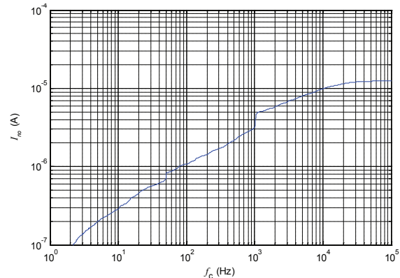
Figure 14: Typical total RMS noise current with R_M = 50 \Omega
