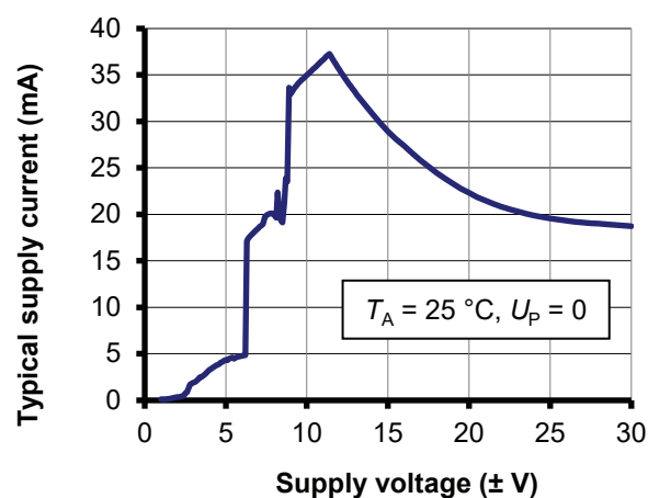
Figure 7: Supply current function of supply voltage
