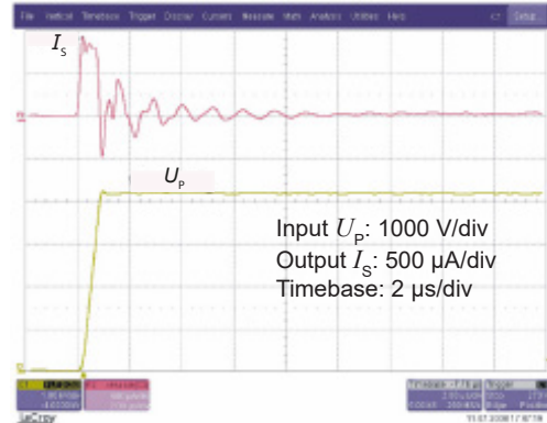
Figure 12: Detail of typical common mode perturbation (4200 V step with 6 kV/μs, R_M = 100 \Omega )
