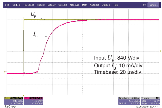
Figure 6: Typical step response (0 to 4200 V)
