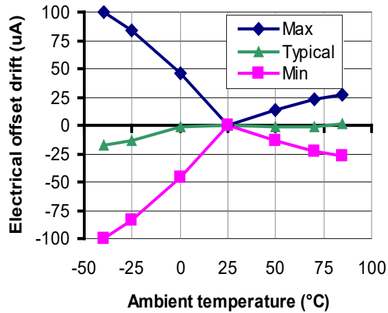
Figure 3: Electrical offset thermal drift
