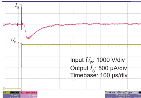
Figure 11: Typical common mode perturbation (4200 V step with 6 kV/μs R_M = 100 \Omega )
