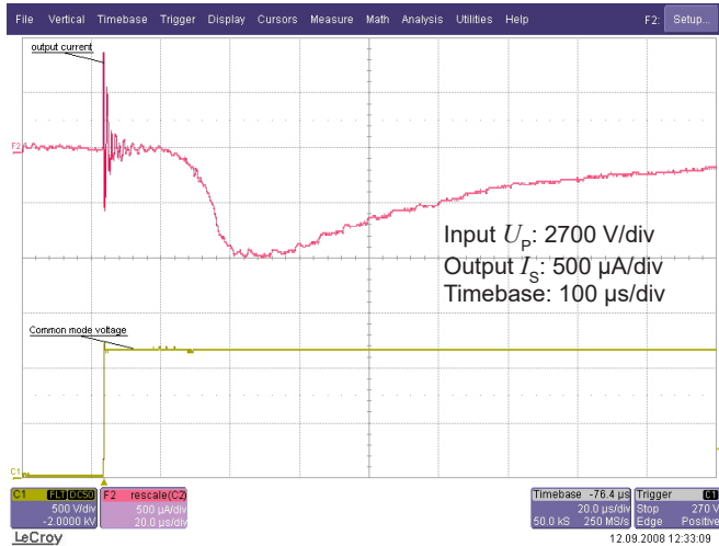
Figure 12: Typical common mode perturbation (6400 V step with 6 kV/µs, R_M = 100 \Omega )
