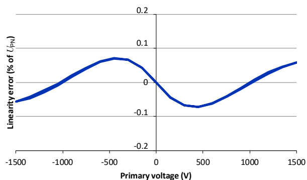
Figure 5: Typical linearity error at 25 °C
