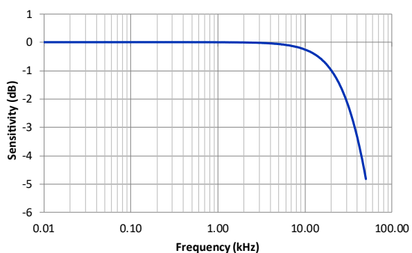
Figure 8: Sensitivity function of frequency
