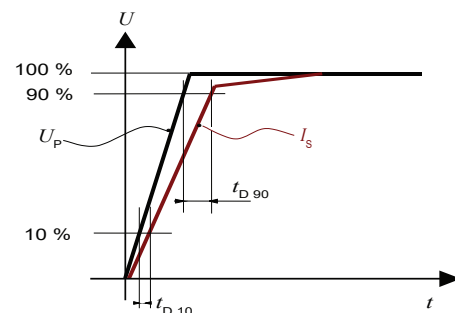
Figure 14: Delay time t_{D10} @ 10 % and delay time t_{D90} @ 90 %.
