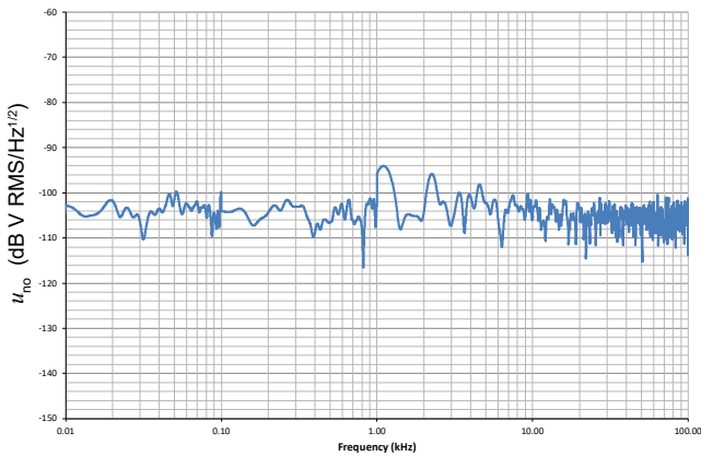
Figure 10: Typical output noise voltage spectral density U_{no} referred to secondary
