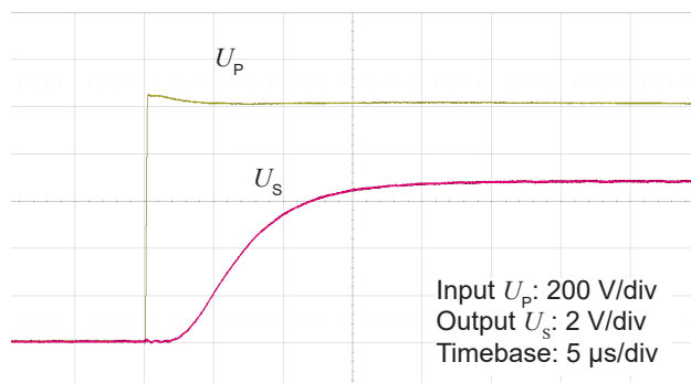
Figure 7: Typical delay time (0 to 1000 V)
