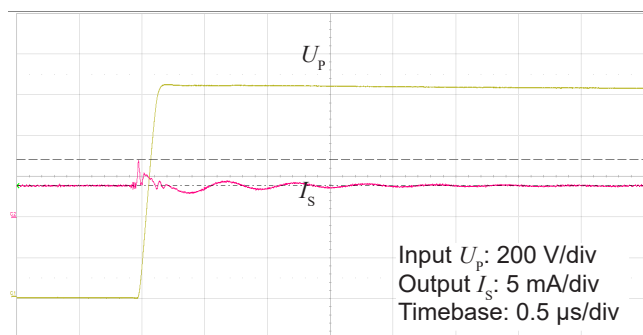
Figure 7: Detail of typical common mode perturbation (1000 V step with 6 kV/ \mu s, R_M = 100 \Omega )
