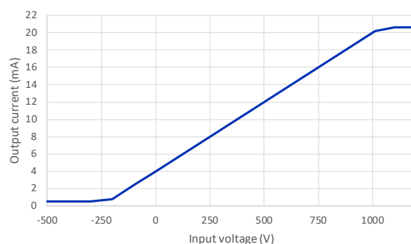
Figure 2: Output secondary current
