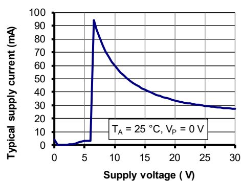
Figure 2: Supply current function of supply voltage
