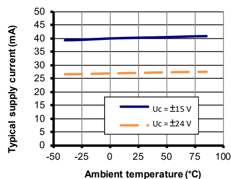
Figure 2: Supply current function of temperature
