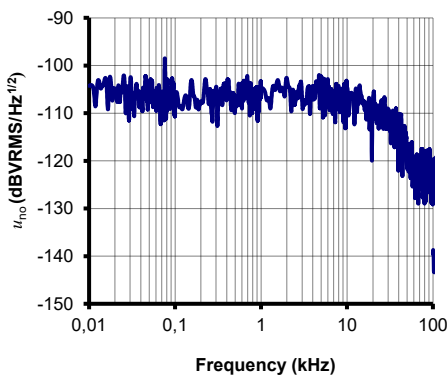
Figure 7: Typical output noise voltage spectral density u_{no} referred to secondary with R_M = 50 \Omega
