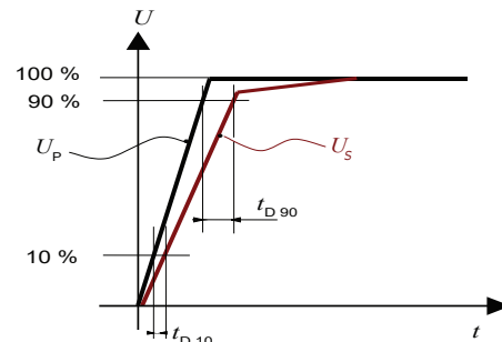
Figure 16: Delay time t_{D10} @ 10 % and delay time t_{D90} @ 90 %.
