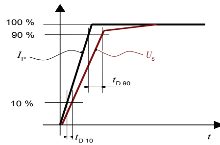
t_{D10} (delay time @ 10 %) and t_{D90} (delay time @ 90 %)
