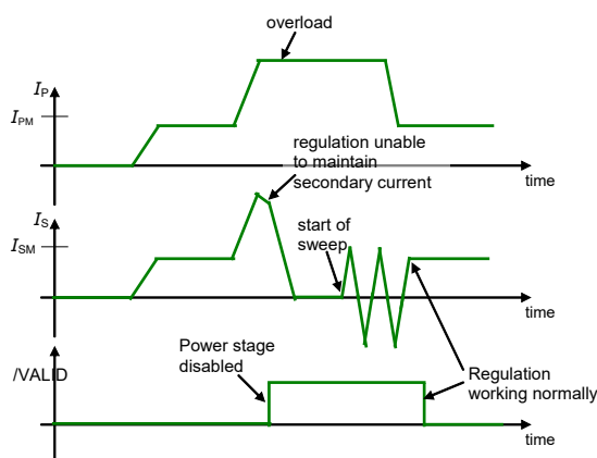
Figure 24: Overload behaviour
