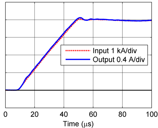
Figure 13: Typical step response (0 to 4 kA, 100 A/μs)
