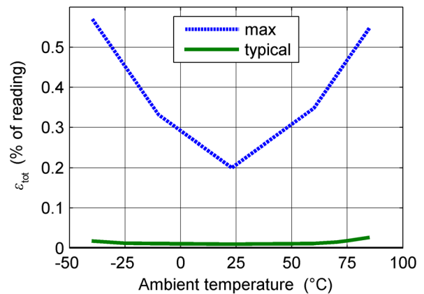
Figure 2: Total error in temperature for 0.1 I_{PN} \leq I_P \leq 1.5 I_{PN}
