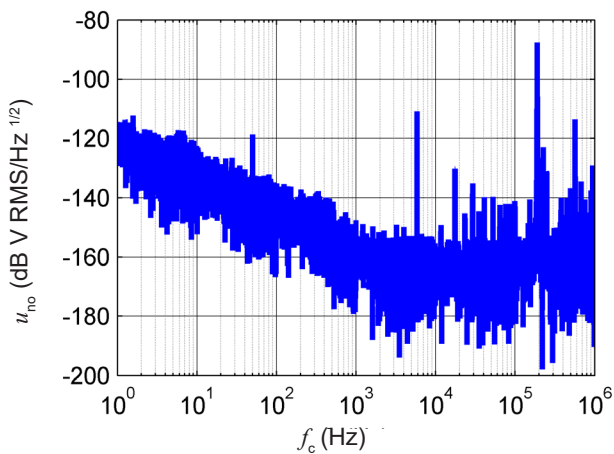
Figure 15: Typical noise voltage spectral density u_{no} with R_M = 1 \Omega
