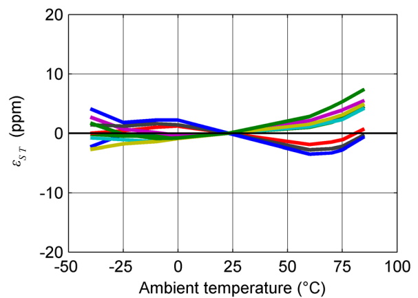
Figure 6: Typical sensitivity variation in temperature (9 samples shown)
