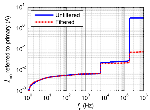
Figure 16: Typical total output noise current (primary referred, RMS) with R_M = 1 \Omega ( f_c is upper cut off frequency of bandpass, low cut off frequency is 1 Hz). Filtered output was measured with 10 kHz 1 st order low pass filter.
