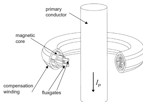
Figure 21: ITC head construction
