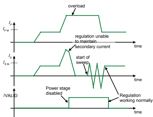
Figure 24: Overload behavior
