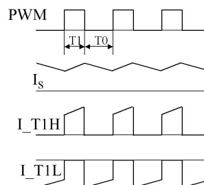
Figure 22: Power stage principle
