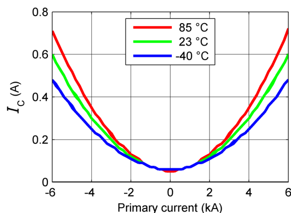
Figure 8: Typical supply current function of primary current ( R_M = 0.1 \Omega , \pm U_C = \pm 24 V) (both supply currents are identical)
