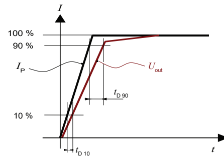
Figure 4: t_{D10} (delay time @ 10 %) and t_{D90} (delay time @ 90 %)
