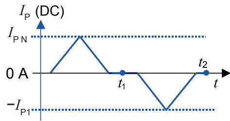
Figure 3: Current cycle used to measure magnetic and electrical offset (transducer supplied)
