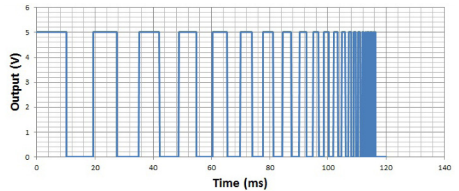
Figure 2: Degauss cycle
